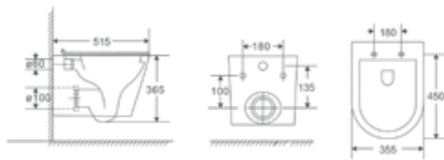
CLEMENT TORNADO FALI RIMLESS WC
